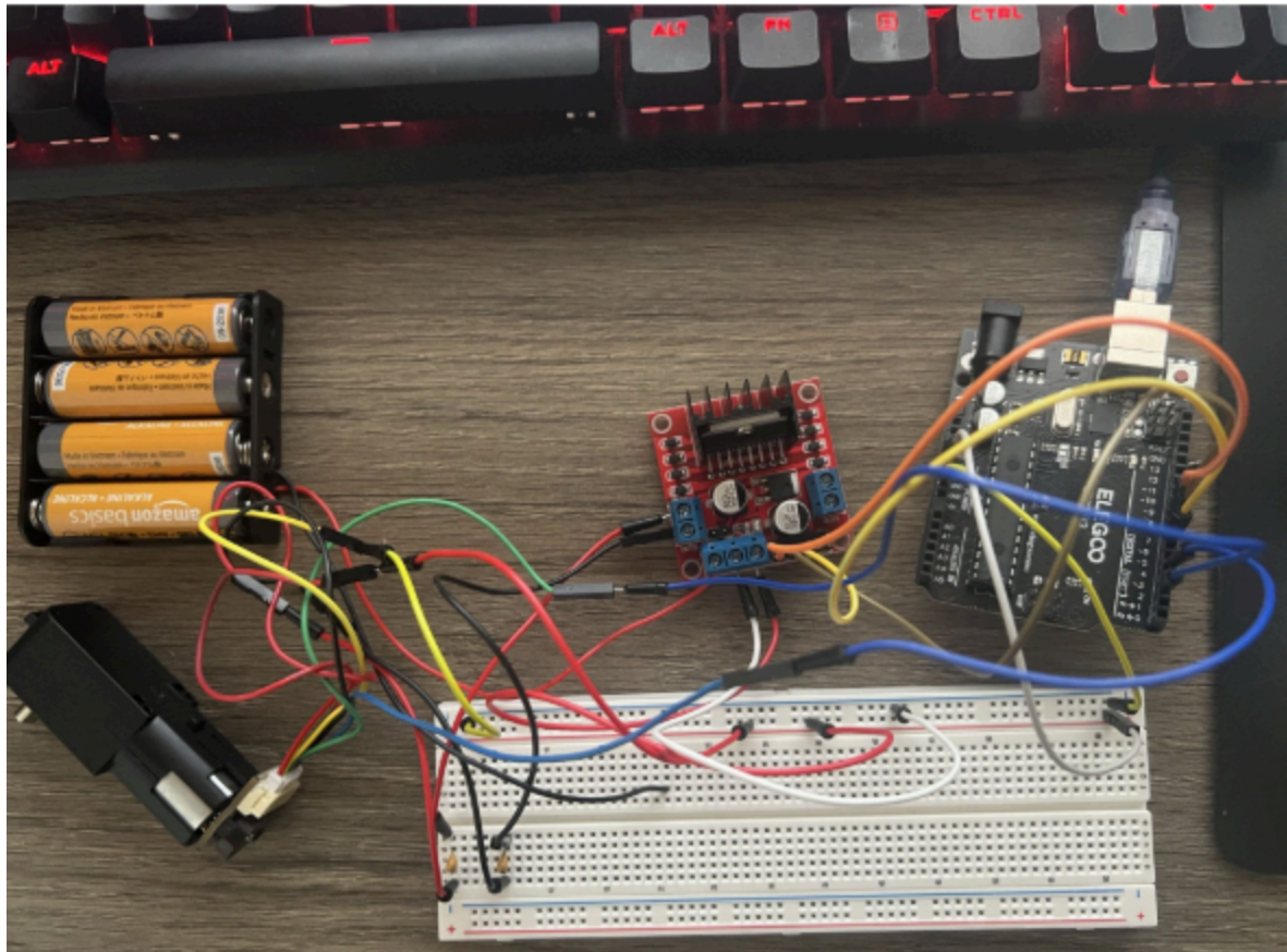
(Figure 1. As-built breadboard setup: Arduino UNO, L298N driver, TT encoder motor, 4×AA pack.)
