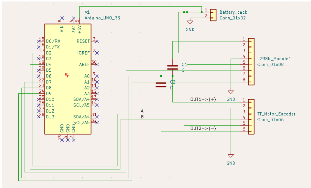
(Figure 2 – Schematic)
